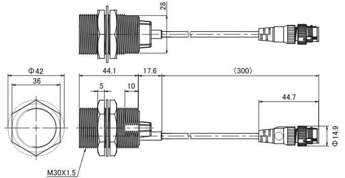
BS-K1117M-M30-3012
